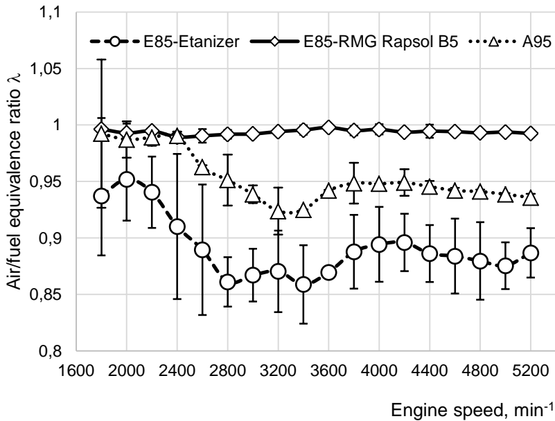
Figure 8. Fuel and conversion kit influence on air-fuel equivalence ratio.
